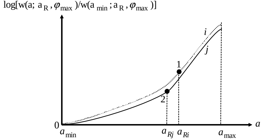
Figure 5: Relative wages in countries i and j , when \bar{\varphi}_i > \bar{\varphi}_j
