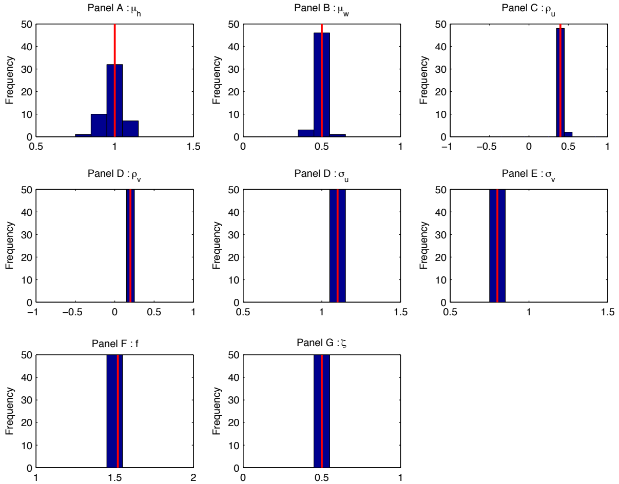
Figure D.1: Monte Carlo Results
